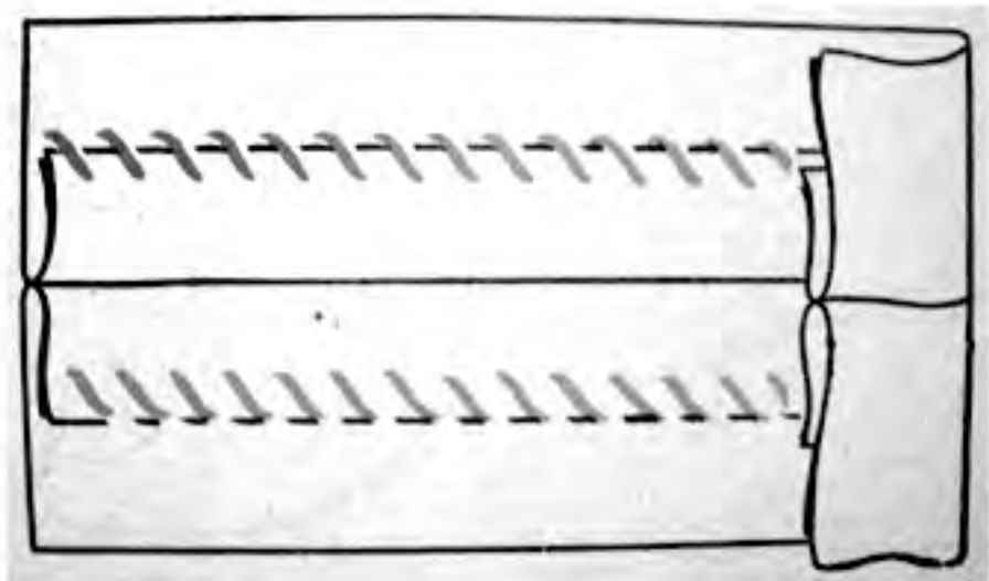
Overcast Seam Finish
